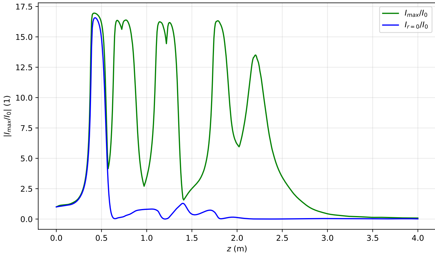
I_{max}(x=0, y=0, z)/I_0 , P_{in}=6.5P_{cr} , noisy input, artificial time
